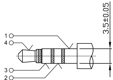
φ3.5 MATE PLUG
