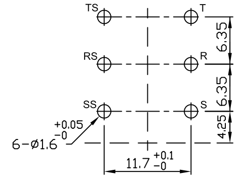
P.C.B LAYOUT (TOP VIEW)(±0.1)
