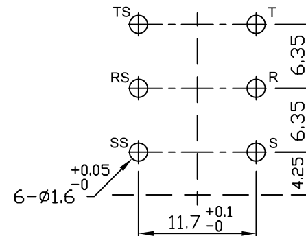
P.C.B LAYOUT (TOP VIEW)(±0.1)
