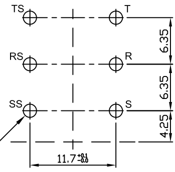
▲ (TOP VIEW) P.C.B LAYOUT ±0.1
